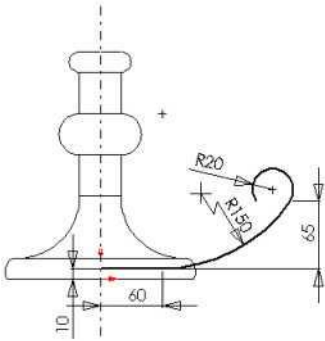
Path, sketch on Front Plane
